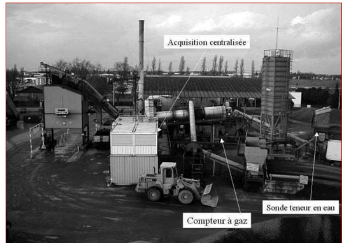
Figure 1: Implantation de l'instrumentation.
